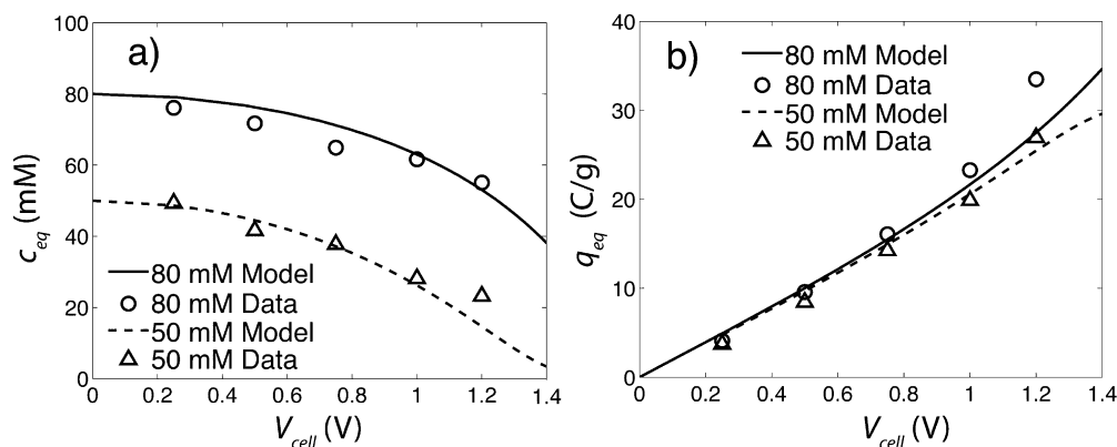
Figure 2. Model result and measured (a) equilibrium salt concentration, c_{eq} , and (b) equilibrium charge stored, q_{eq} , vs applied potential for initial salt concentrations of 50 and 80 mM. Measured data for c_{eq} is obtained from visualizations and q_{eq} from current measured for the two-electrode cell. The model lines are obtained from the modified Donnan (mD) model results.
