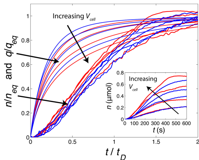
Figure 4. (a) Measurements of normalized salt removed from the visualized space between electrodes, n/n_{eq} and normalized charge stored, q/q_{eq} versus time nondimensionalized by the diffusion time across the separator half-width, t/t_D . Data includes results for initial concentrations of 80 mM (blue lines) and 50 mM KCl (red lines) and voltages of 0.5, 0.75, 1, and 1.25 V. Voltage is applied at t = 0 s. Normalizing n by n_{eq} causes an approximate collapse of these curves (see the dimensional data in the inset). Further, distinct differences are observed between the nondimensional cell charging ( q/q_{eq} ) and desalination ( n/n_{eq} ) dynamics. The cell charges quickly upon application of the electric field, reaching roughly 50% charged at a time of 0.25. Desalination requires longer times, as the space between electrodes is roughly only 10% desalted at a time of 0.25. Significant desalination occurs at times of approximately unity (the diffusion time), as n/n_{eq} \cong 0.6 at t/t_D \cong 1 .
